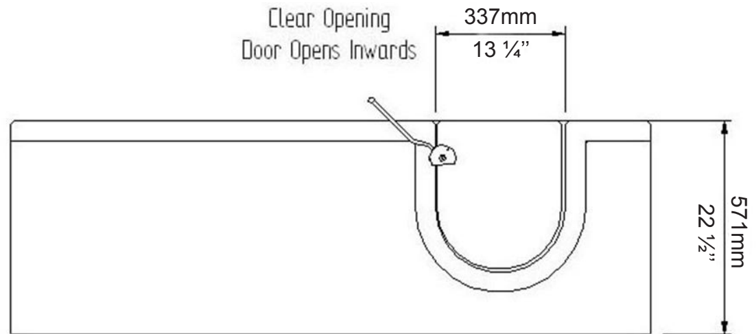
Front Elevation
